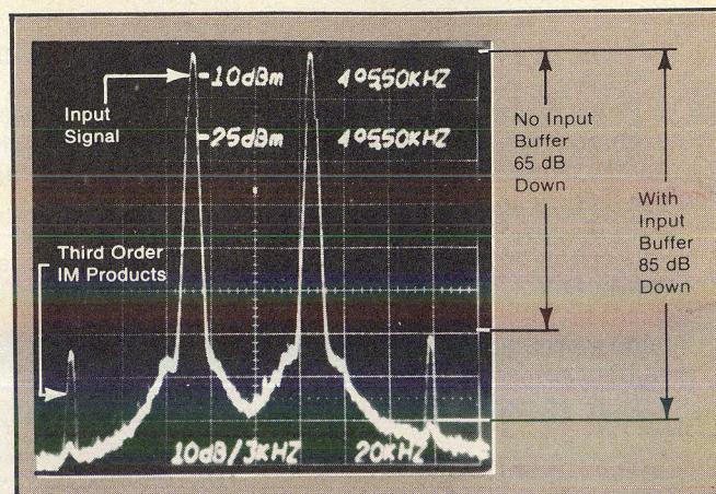
2. An input attenuator circuit that proportionally increases instrument gain to balance loss can reduce third-order IM products and thereby increase dynamic range.
