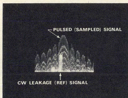
7. IF gating method allows a small level of CW leakage that can be used as a reference.
