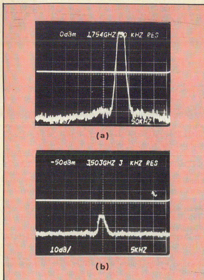
3. Tracking preselectors reject the fundamental while the spectrum analyzer tunes to the second harmonic; self-generated harmonics thus do not interfere with the measurement. Here, the fundamental is displayed at -5 dBm (a), while the second harmonic, at -100 dBm, is down by 95 dB (b).
