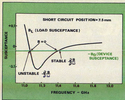
6. Stable and unstable regions are determined by plotting load and device susceptance and evaluating their relative magnitudes
