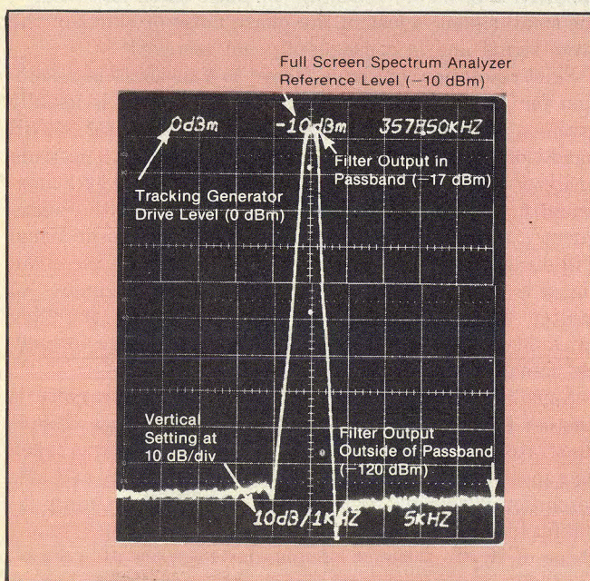
4. High ultimate attenuation measurement using a tracking generator shows over 100-dB of out-of-band rejection.
