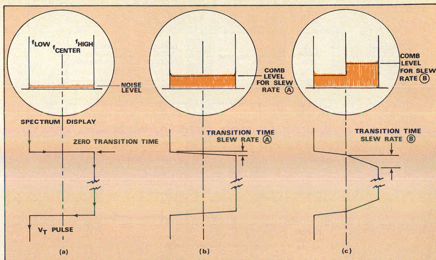
11. Magnitude of combline spectrum displayed on the spectrum analyzer CRT is larger for slower tuning slew rates.
