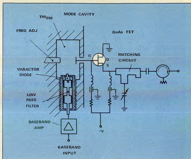
3. A grounded-drain GaAs FET (Fujitsu FLC-15) is at the heart of this 7-GHz FM modulator.
