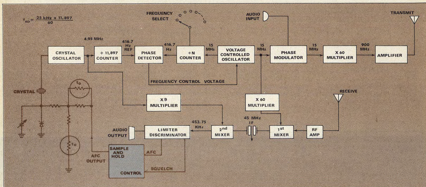
8. This duplex mobile radio design incorporates memory to use base-station stability as a reference. Stabilizing circuit is shown in color.
