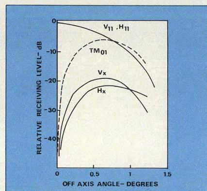
2. The received TM_{01} mode is useful for adjusting antenna direction to maximize cross-polarization discrimination.
